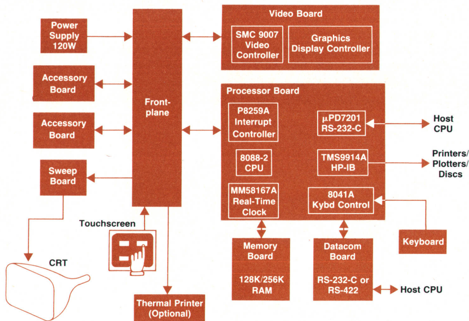
Fig. 2. HP 150 hardware block diagram. The CPU is an 8088 microprocessor running at 8 MHz.
