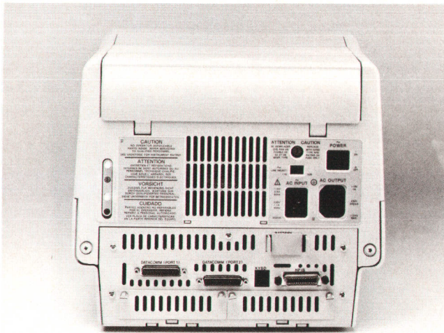
Fig. 2. The rear panel of the HP 150 has three I/O ports and two slots (behind slotted panels at the bottom) for hardware options.
